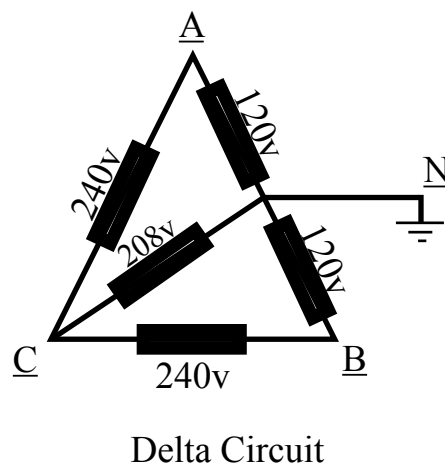
Figure 11. Delta Winding Connections
