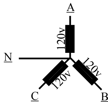
Star Circuit
